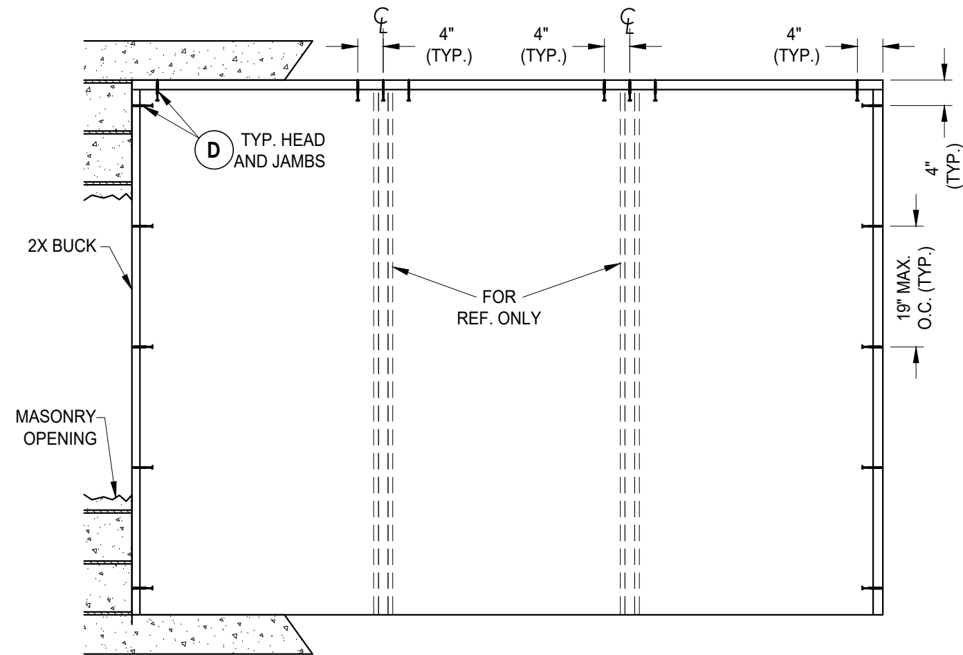
BUCK ANCHORING
