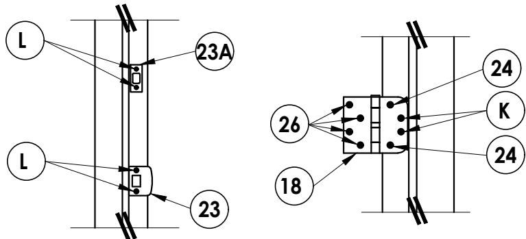
STRIKE PLATE DETAIL
